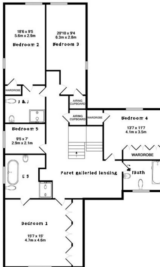
1ST FLOOR APPROX. FLOOR AREA 1450 SQ.FT. (134.7 SQ.M.)
