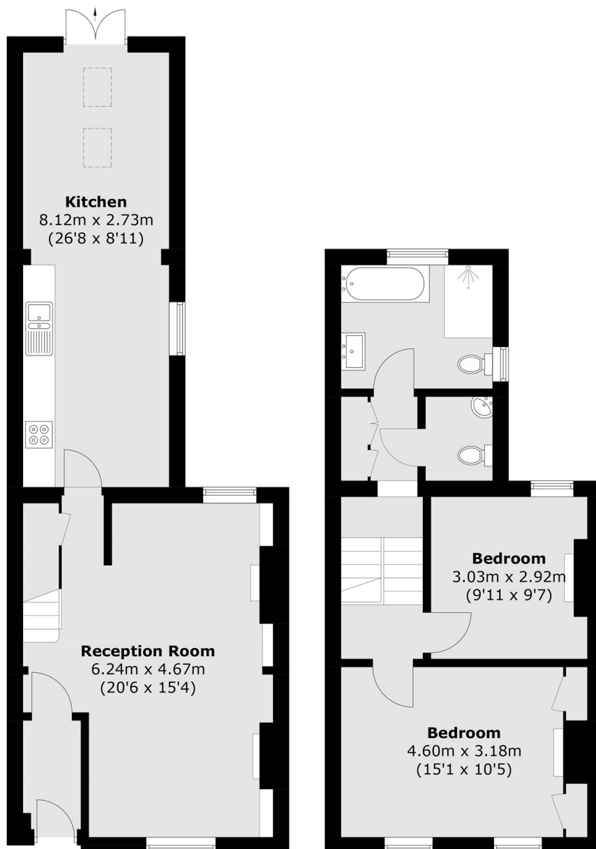
Ground Floor
