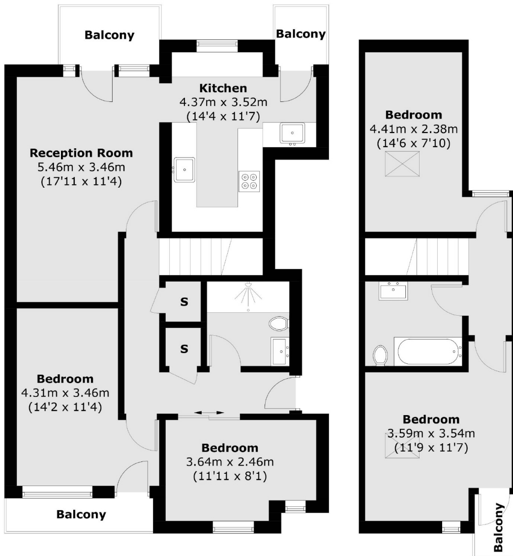
Third Floor
