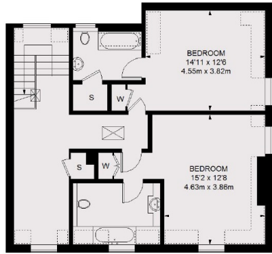
THIRD FLOOR
