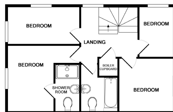
1ST FLOOR APPROX. FLOOR AREA 539 SQ.FT. (50.1 SQ.M.)
